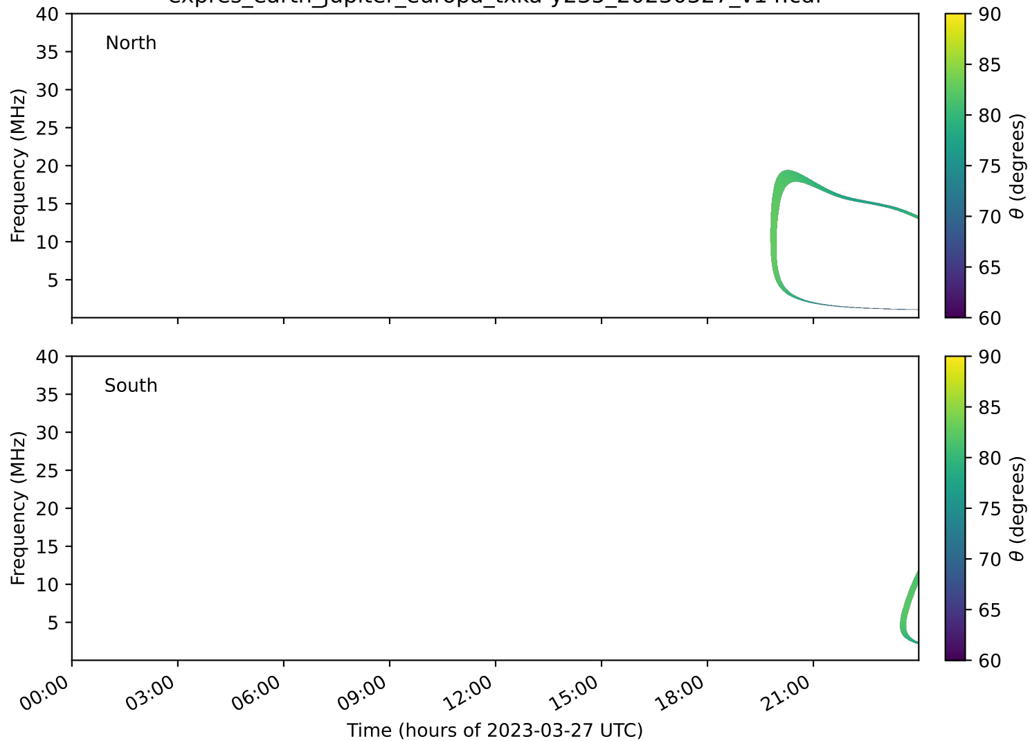
expres_earth_jupiter_europa_txka-y235_20230327_v14.cdf
