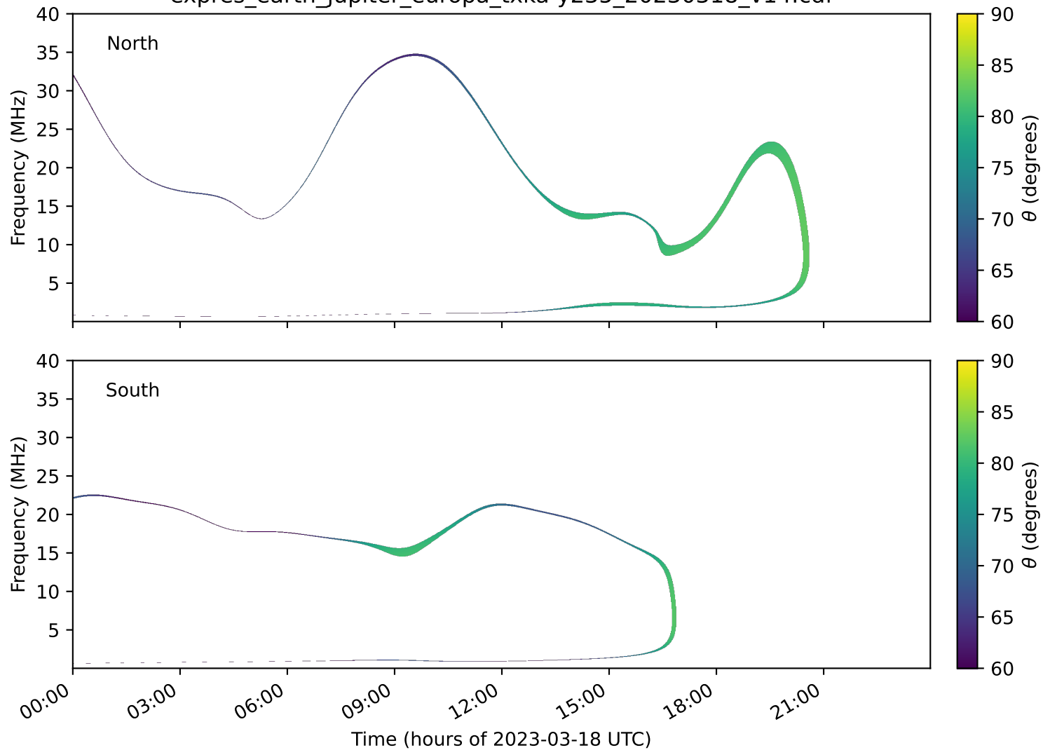
expres_earth_jupiter_europa_txka-y235_20230318_v14.cdf
