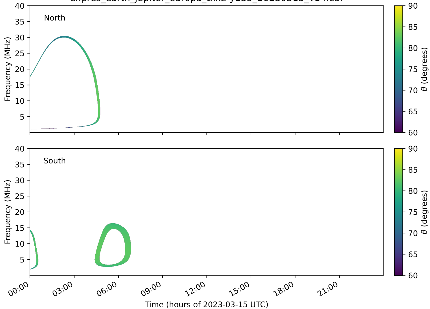
expres_earth_jupiter_europa_txka-y235_20230315_v14.cdf
