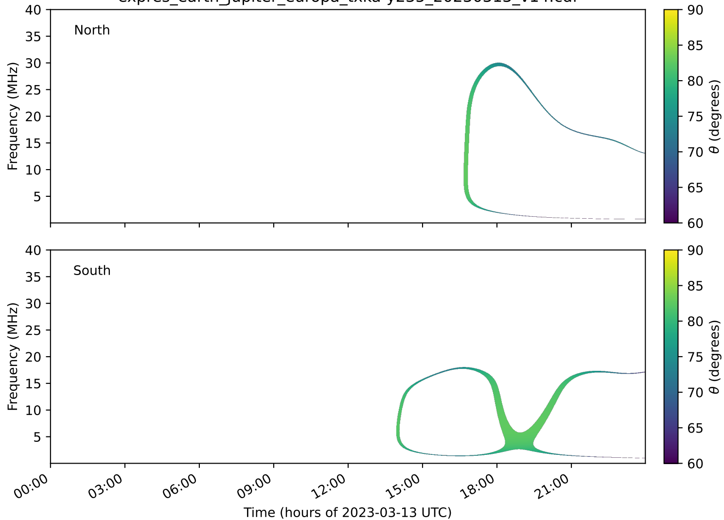
expres_earth_jupiter_europa_txka-y235_20230313_v14.cdf
