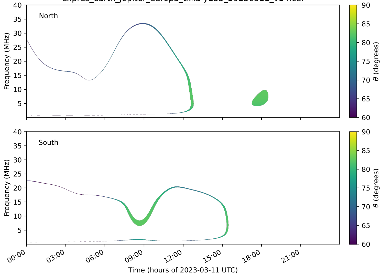
expres_earth_jupiter_europa_txka-y235_20230311_v14.cdf
