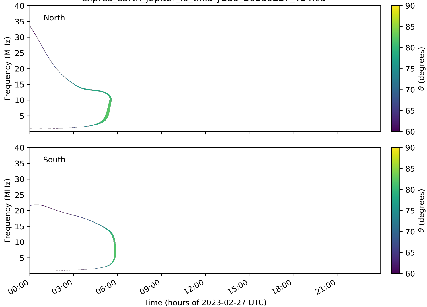
expres_earth_jupiter_io_txka-y235_20230227_v14.cdf
