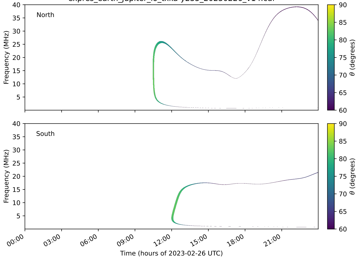
expres_earth_jupiter_io_txka-y235_20230226_v14.cdf
