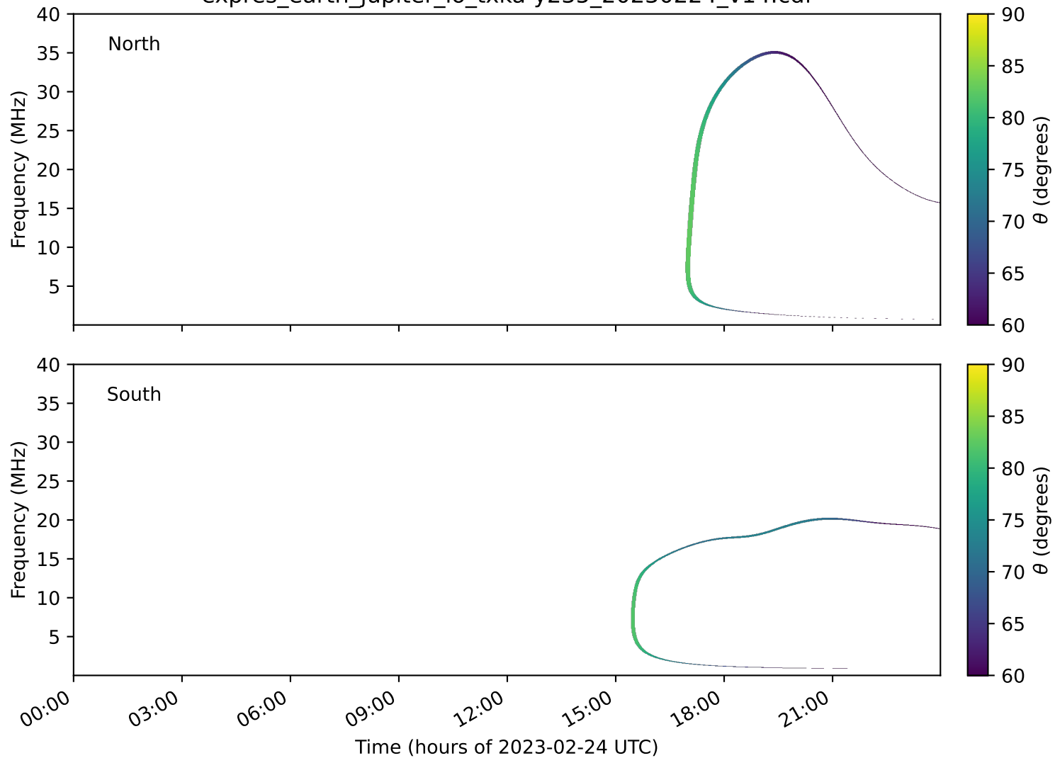
expres_earth_jupiter_io_txka-y235_20230224_v14.cdf
