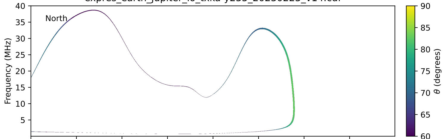
expres_earth_jupiter_io_txka-y235_20230223_v14.cdf
