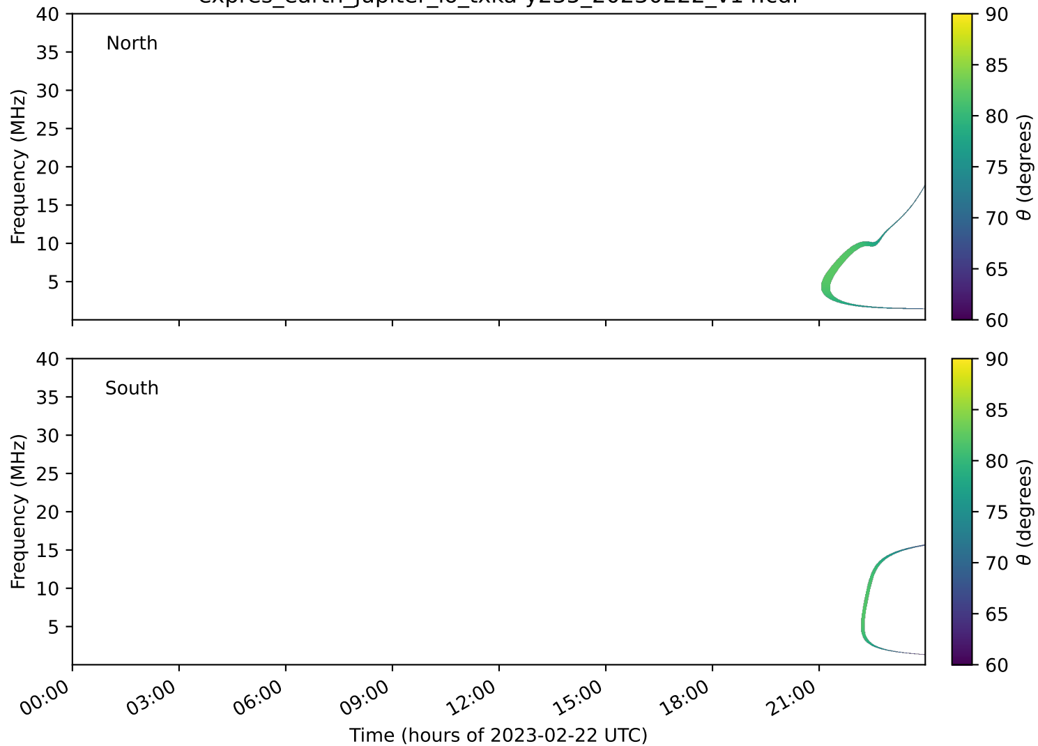
expres_earth_jupiter_io_txka-y235_20230222_v14.cdf
