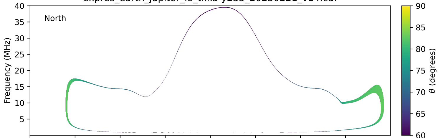
expres_earth_jupiter_io_txka-y235_20230221_v14.cdf
