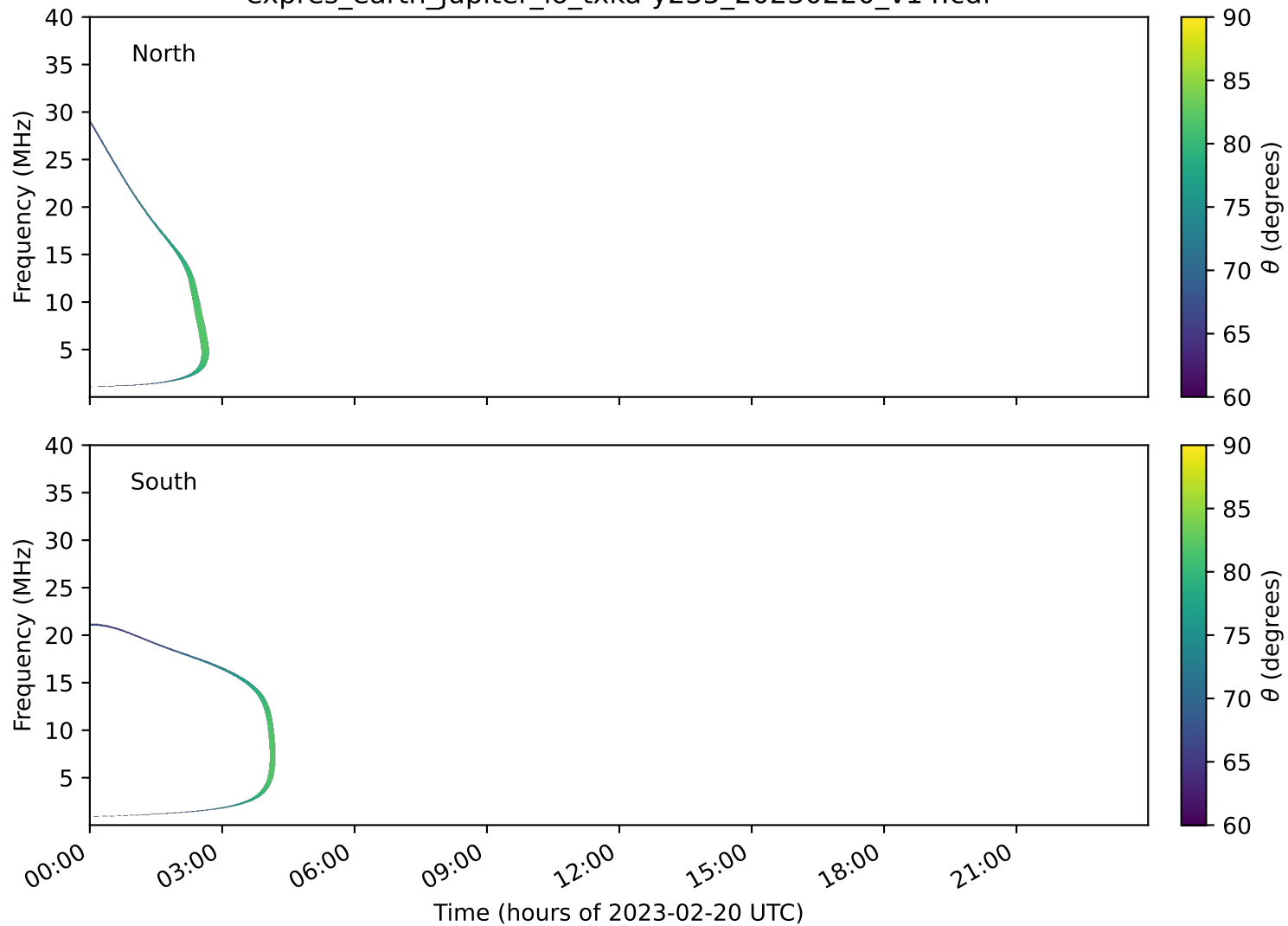
expres_earth_jupiter_io_txka-y235_20230220_v14.cdf
