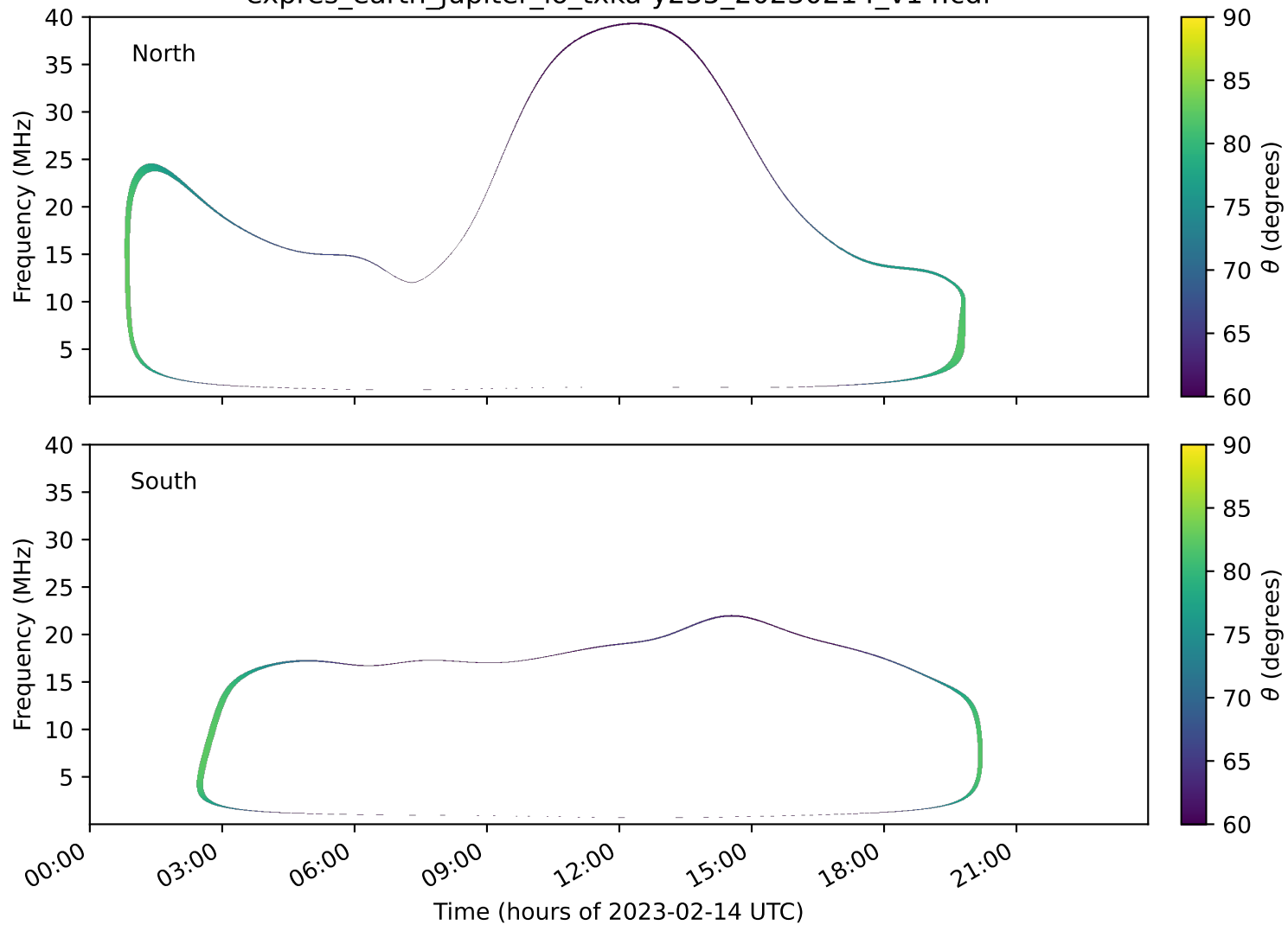
expres_earth_jupiter_io_txka-y235_20230214_v14.cdf
