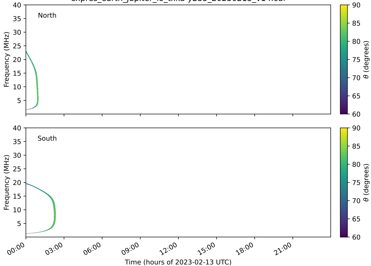
expres_earth_jupiter_io_txka-y235_20230213_v14.cdf
