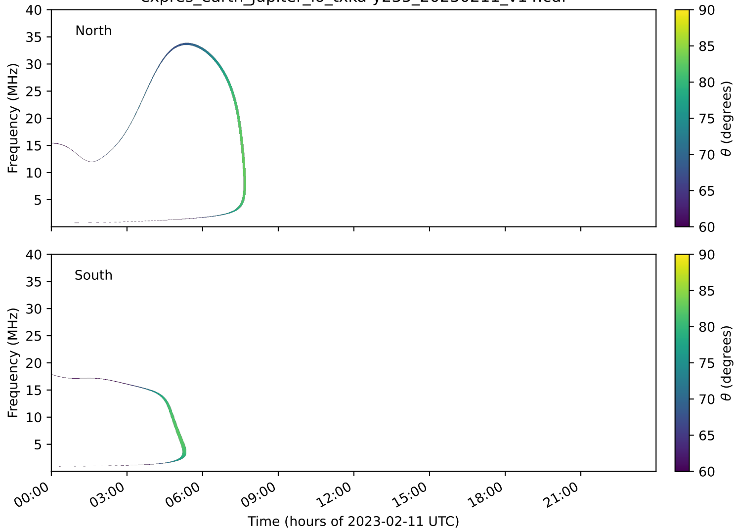
expres_earth_jupiter_io_txka-y235_20230211_v14.cdf
