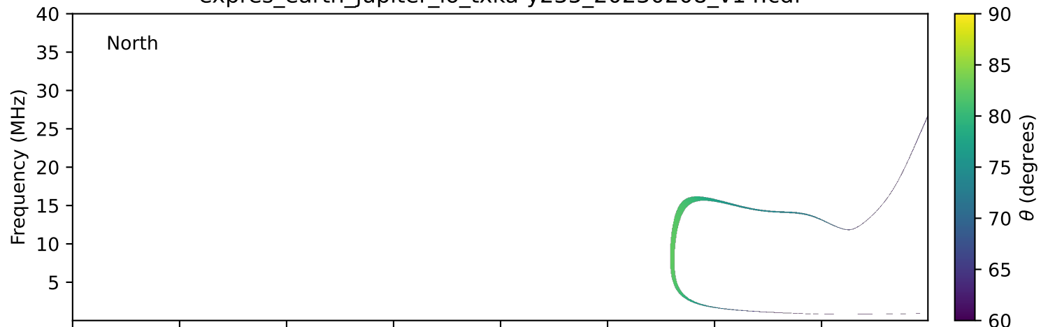
expres_earth_jupiter_io_txka-y235_20230208_v14.cdf
