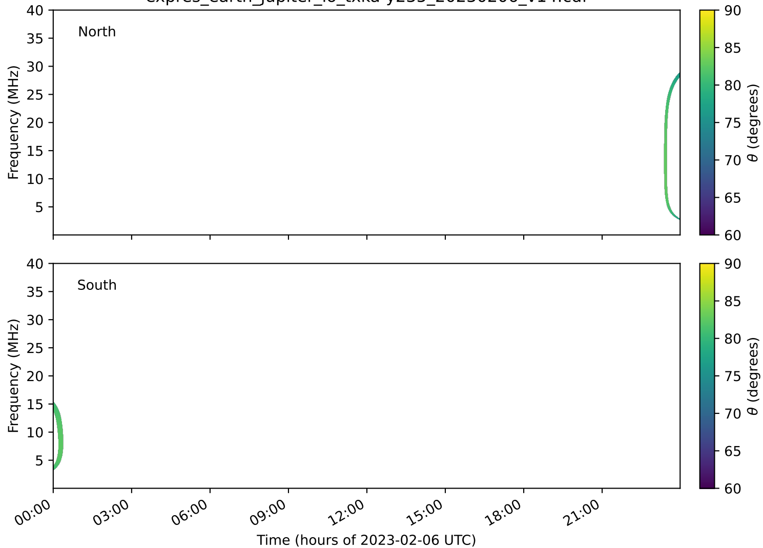
expres_earth_jupiter_io_txka-y235_20230206_v14.cdf
