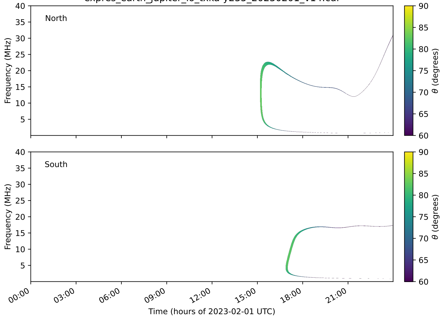
expres_earth_jupiter_io_txka-y235_20230201_v14.cdf
