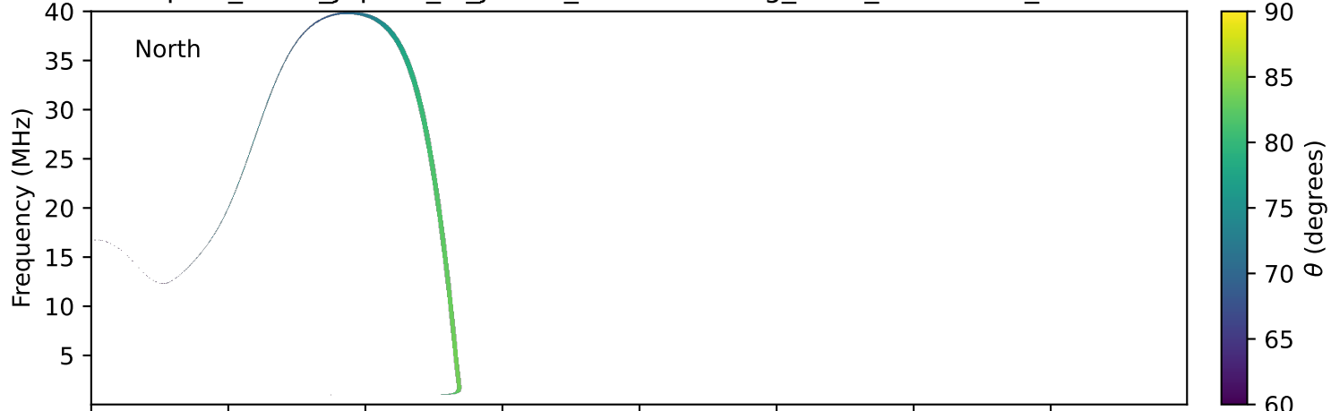
expres_earth_jupiter_io_jrm33_lossc-wid1deg_3kev_20230211_v11.cdf
