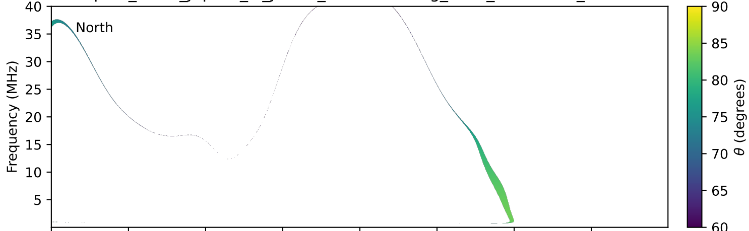
expres_earth_jupiter_io_jrm33_lossc-wid1deg_3kev_20230207_v11.cdf
