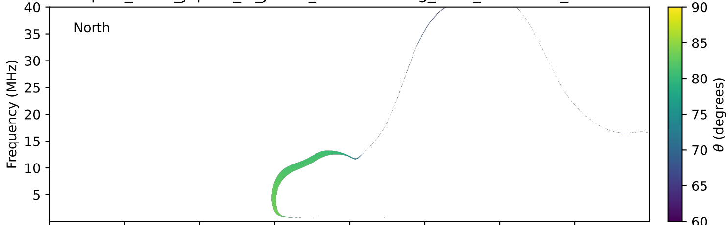
expres_earth_jupiter_io_jrm33_lossc-wid1deg_3kev_20230203_v11.cdf
