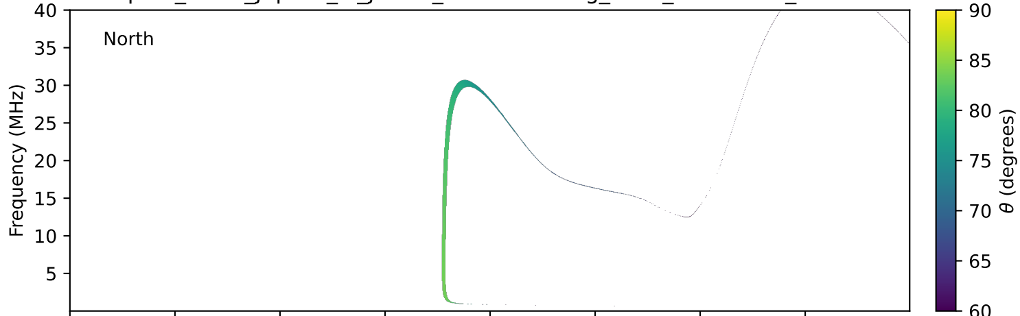
expres_earth_jupiter_io_jrm09_lossc-wid1deg_3kev_20230226_v11.cdf
