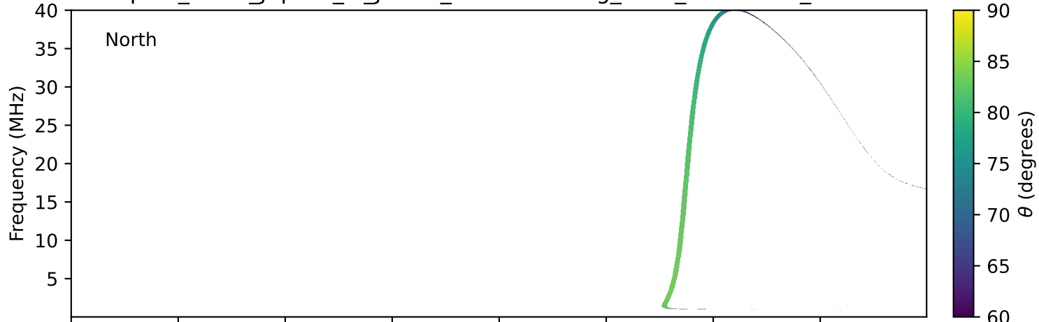
expres_earth_jupiter_io_jrm09_lossc-wid1deg_3kev_20230224_v11.cdf
