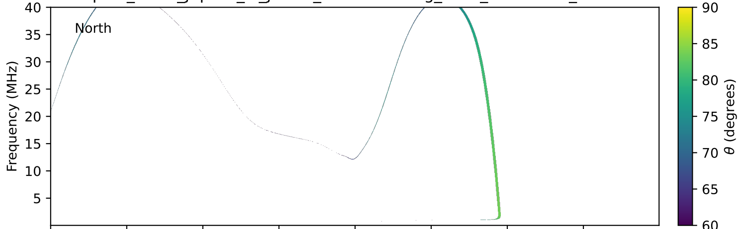
expres_earth_jupiter_io_jrm09_lossc-wid1deg_3kev_20230223_v11.cdf
