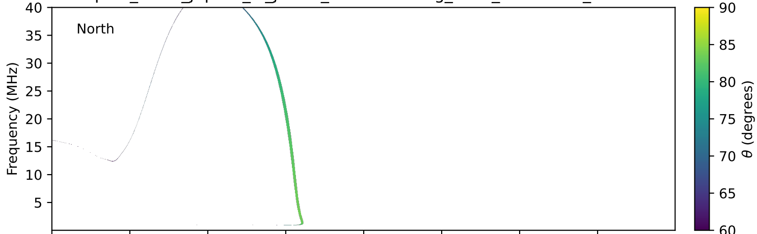
expres_earth_jupiter_io_jrm09_lossc-wid1deg_3kev_20230218_v11.cdf
