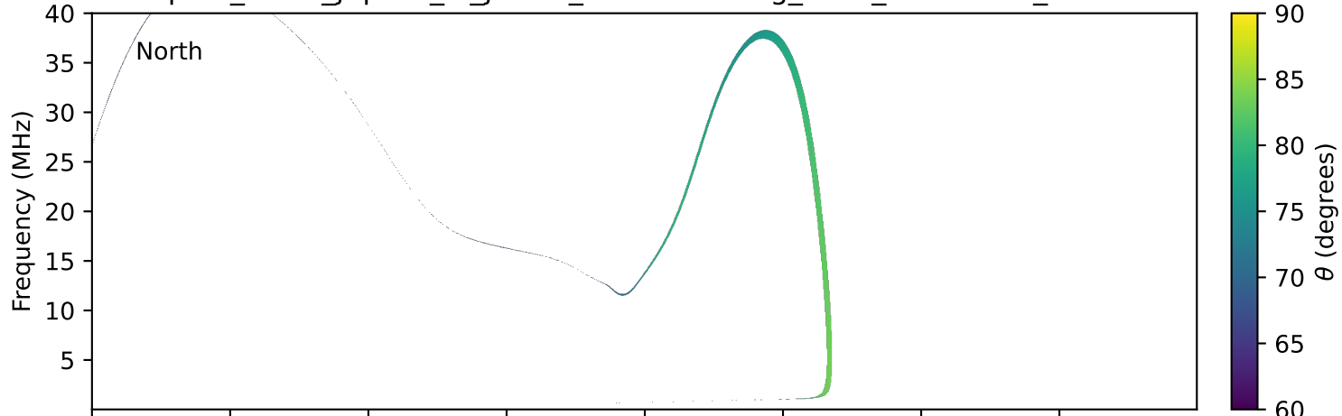
expres_earth_jupiter_io_jrm09_lossc-wid1deg_3kev_20230216_v11.cdf
