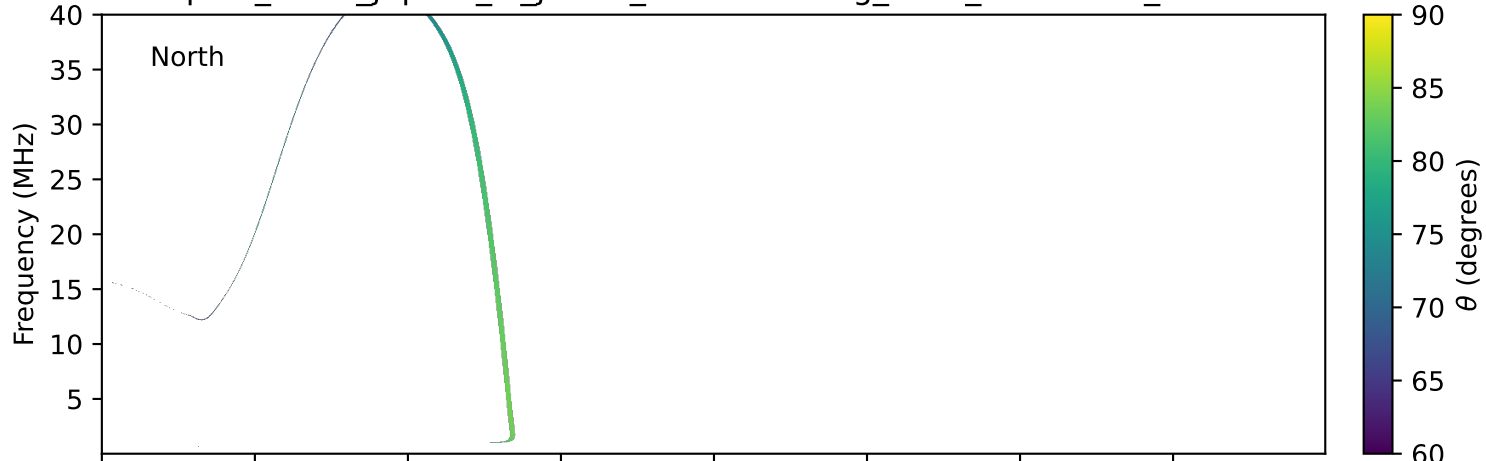
expres_earth_jupiter_io_jrm09_lossc-wid1deg_3kev_20230211_v11.cdf
