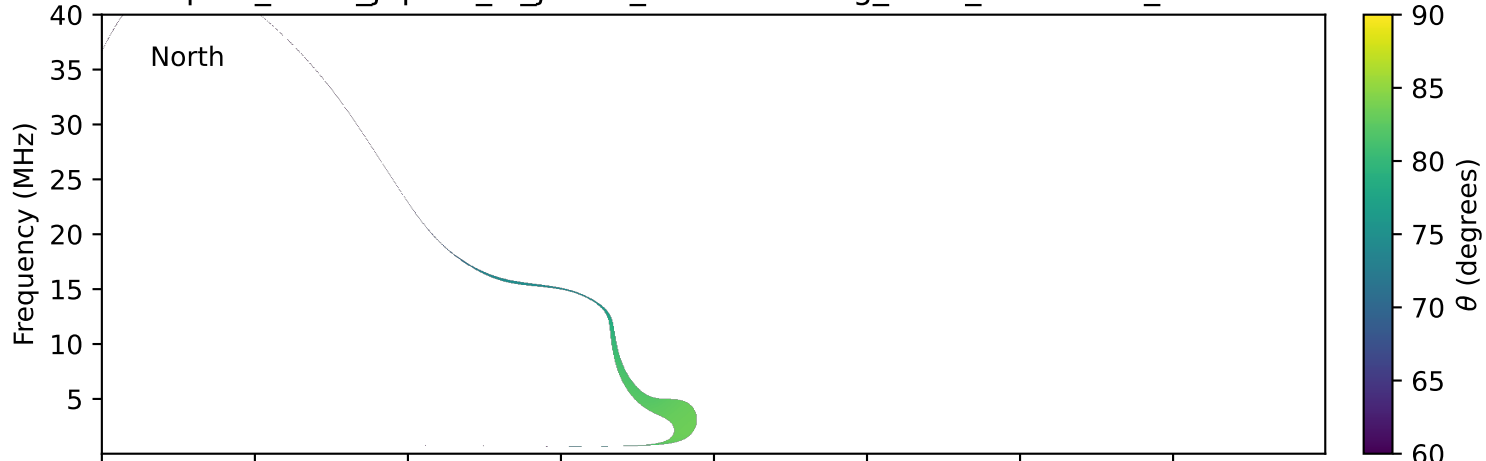
expres_earth_jupiter_io_jrm09_lossc-wid1deg_3kev_20230202_v11.cdf
