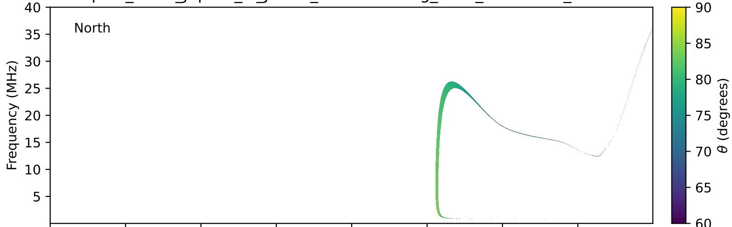
expres_earth_jupiter_io_jrm09_lossc-wid1deg_3kev_20230201_v11.cdf
