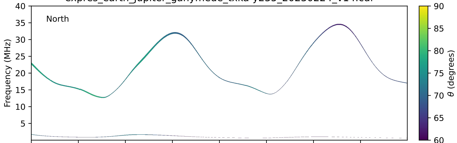
expres_earth_jupiter_ganymede_txka-y235_20230224_v14.cdf
