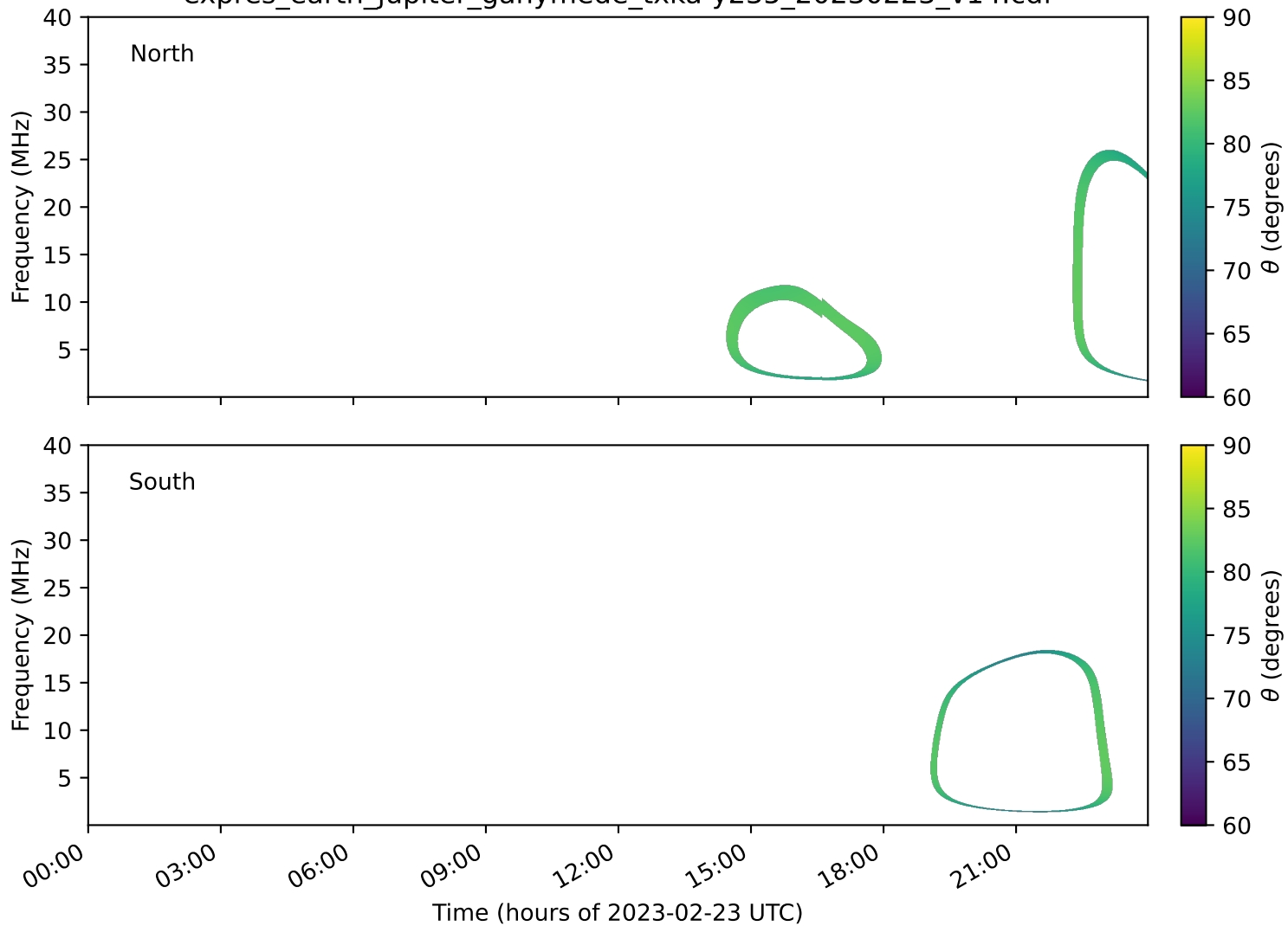
expres_earth_jupiter_ganymede_txka-y235_20230223_v14.cdf
