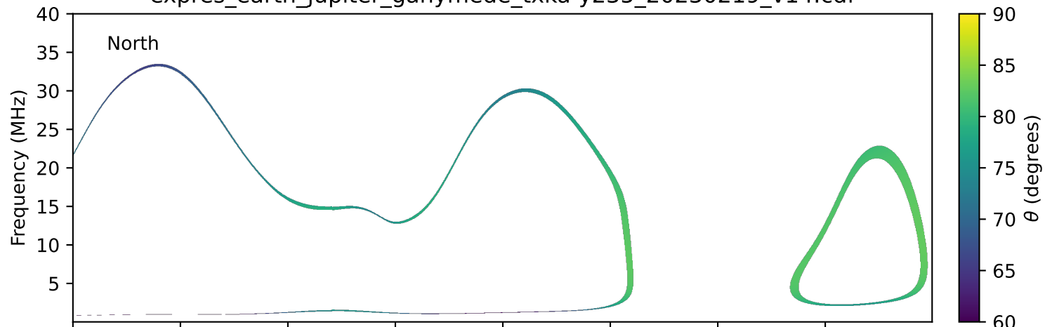
expres_earth_jupiter_ganymede_txka-y235_20230219_v14.cdf
