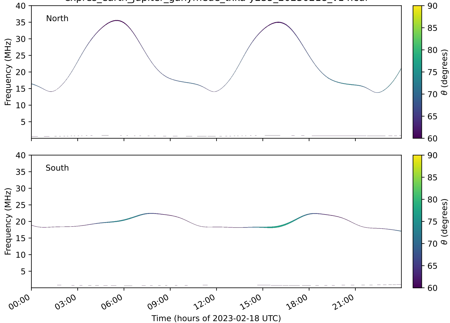
expres_earth_jupiter_ganymede_txka-y235_20230218_v14.cdf
