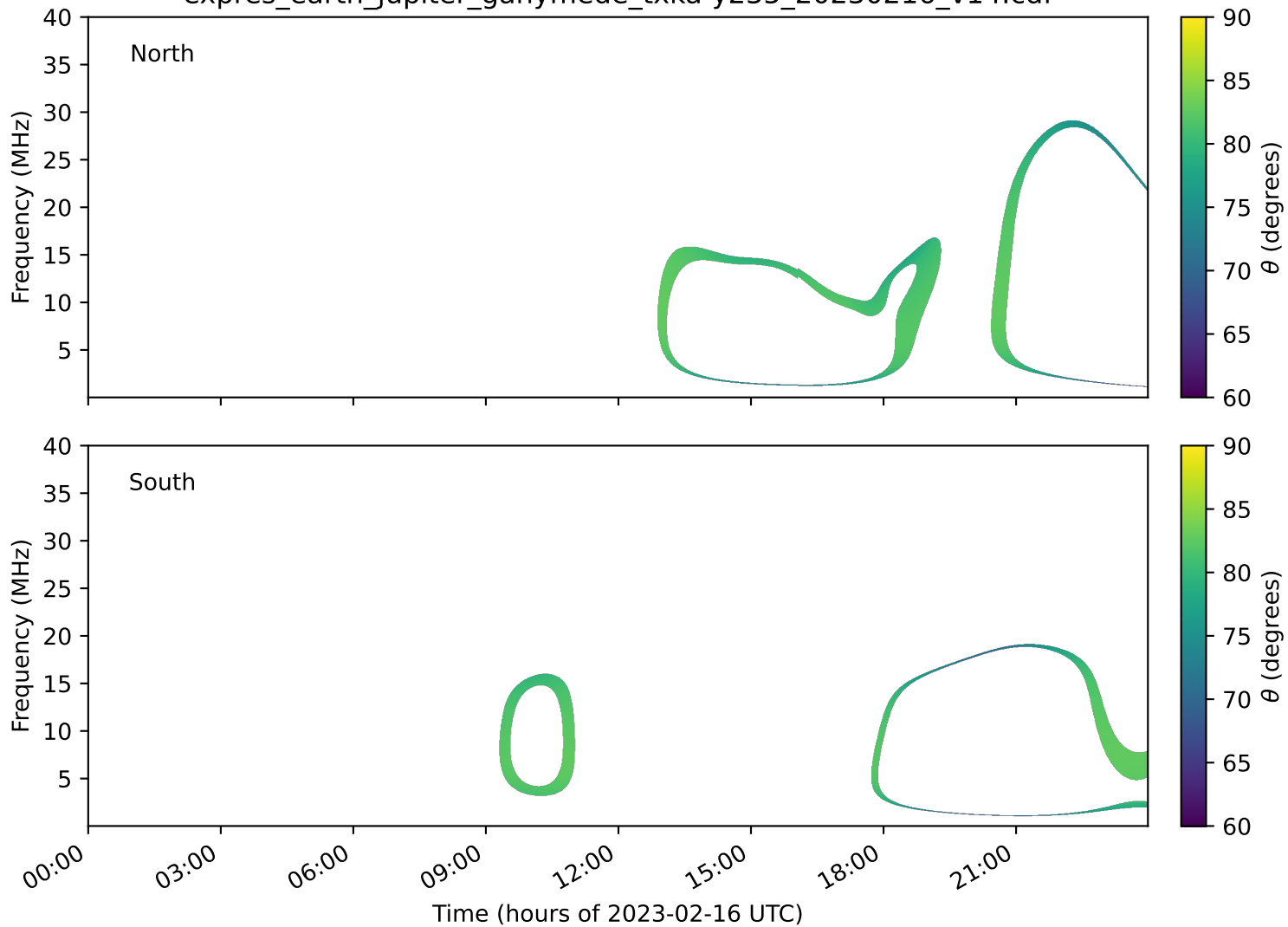
expres_earth_jupiter_ganymede_txka-y235_20230216_v14.cdf
