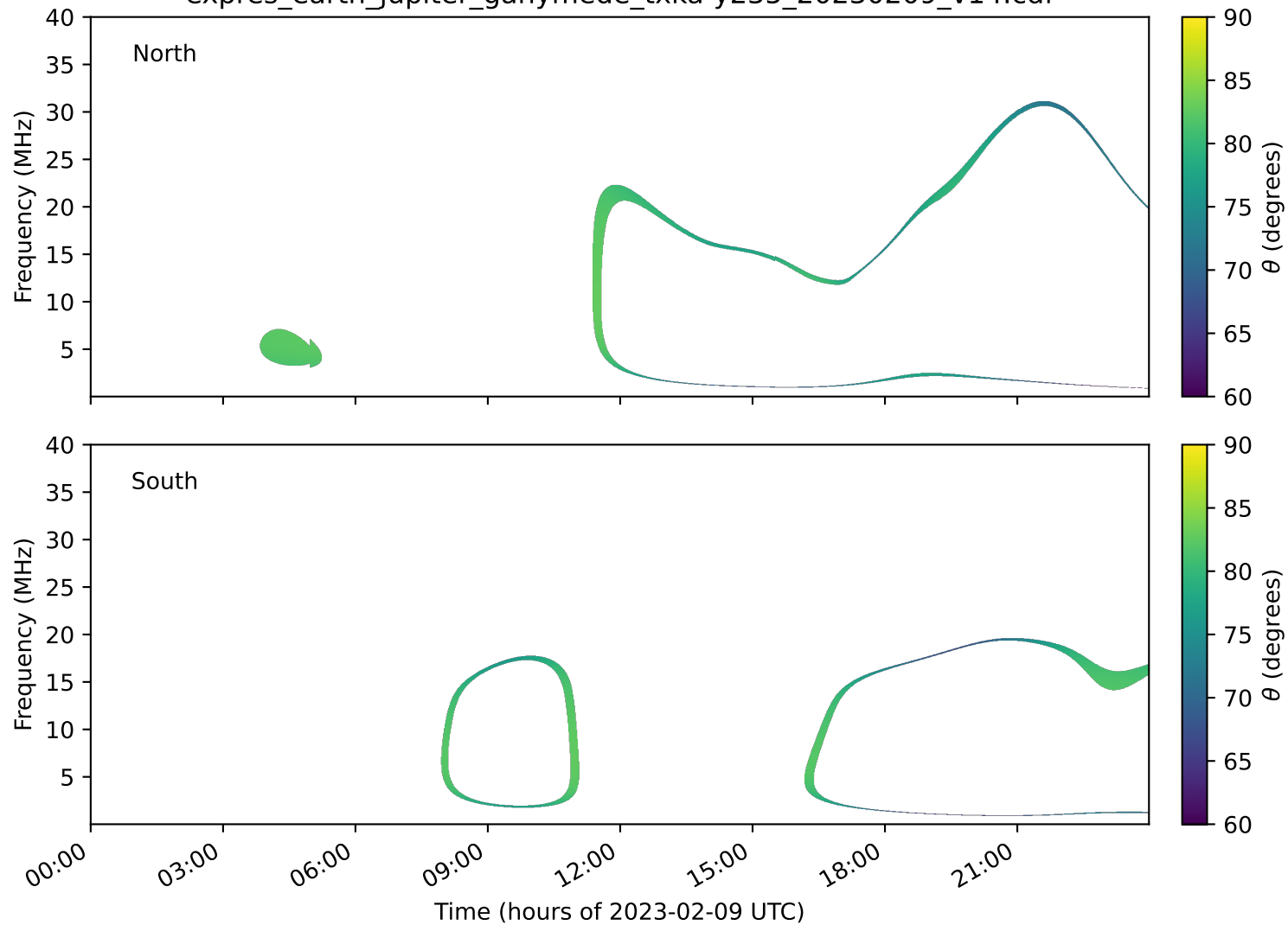
expres_earth_jupiter_ganymede_txka-y235_20230209_v14.cdf
