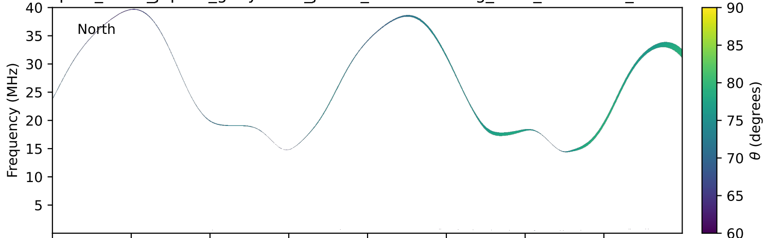
expres_earth_jupiter_ganymede_jrm33_lossc-wid1deg_3kev_20230226_v11.cdf
