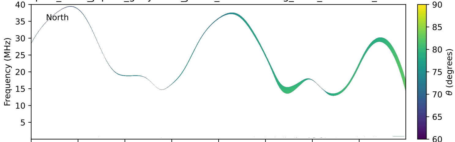
expres_earth_jupiter_ganymede_jrm33_lossc-wid1deg_3kev_20230219_v11.cdf
