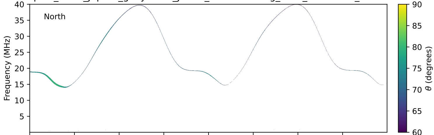
expres_earth_jupiter_ganymede_jrm33_lossc-wid1deg_3kev_20230203_v11.cdf
