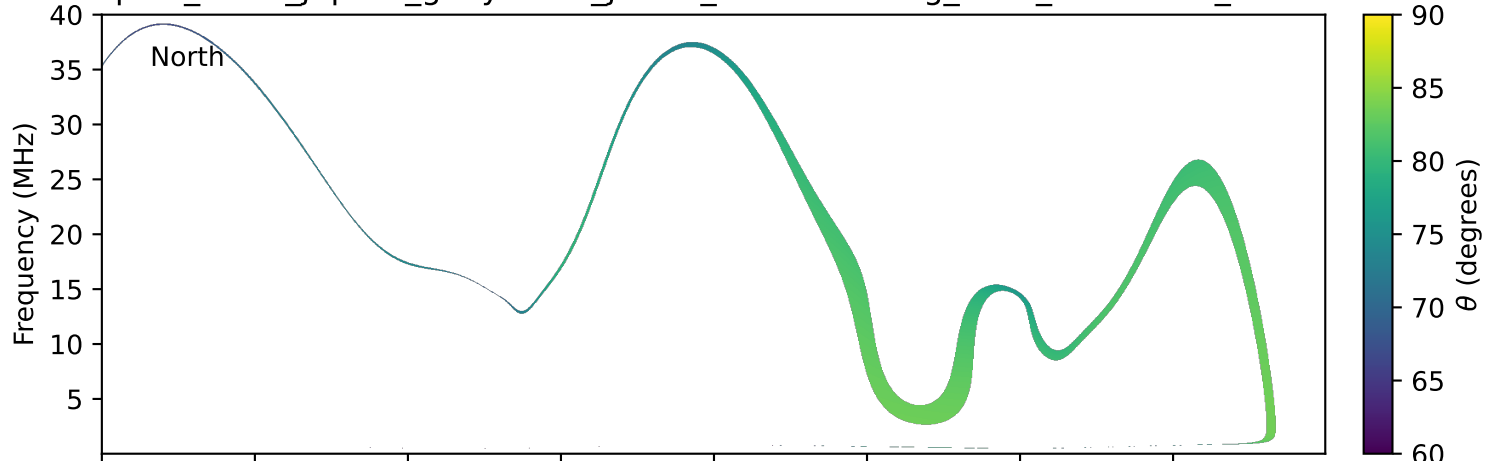
expres_earth_jupiter_ganymede_jrm09_lossc-wid1deg_3kev_20230212_v11.cdf
