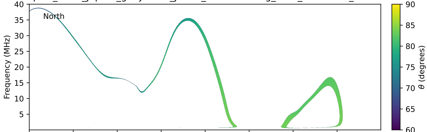
expres_earth_jupiter_ganymede_jrm09_lossc-wid1deg_3kev_20230205_v11.cdf
