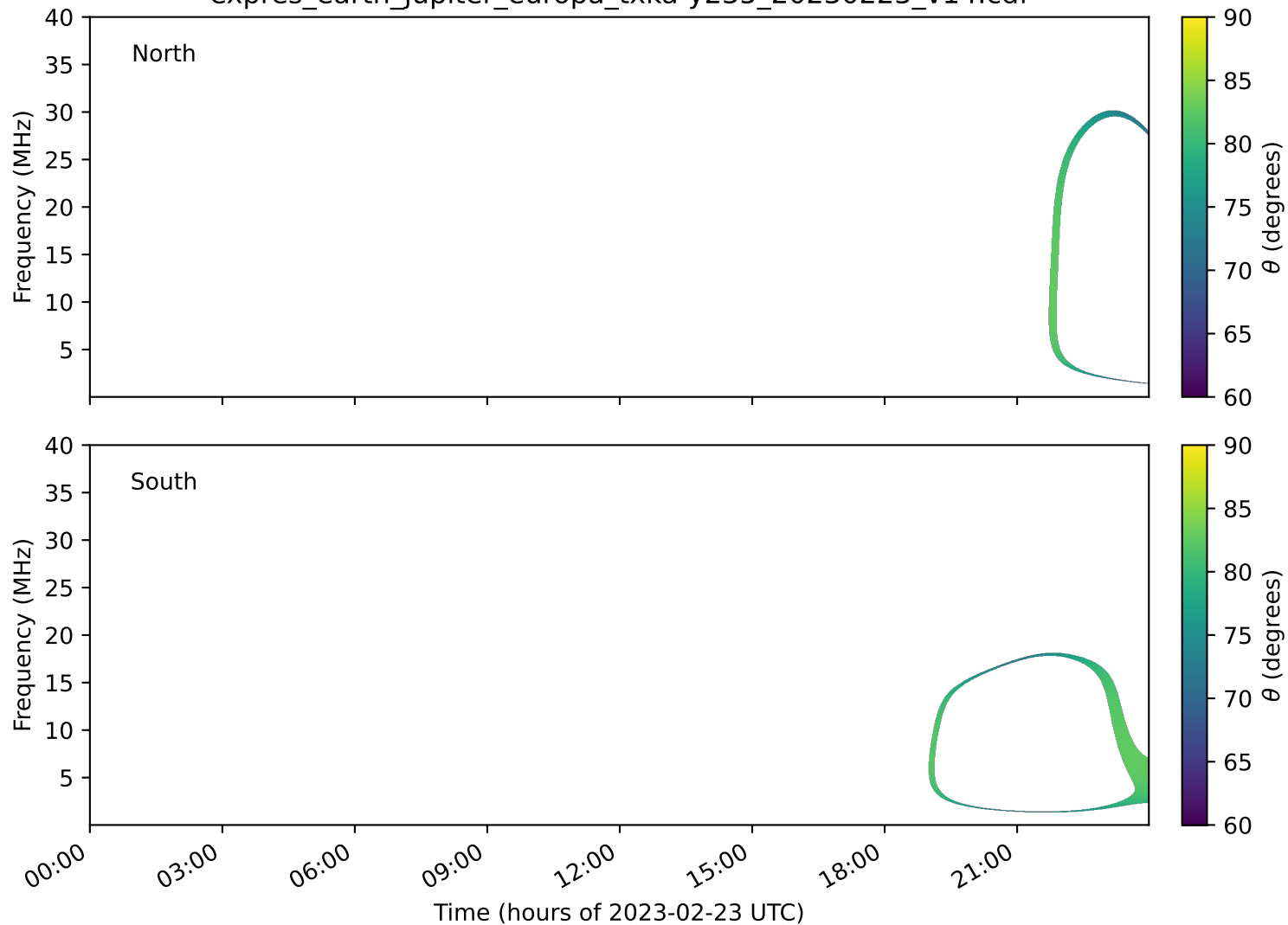
expres_earth_jupiter_europa_txka-y235_20230223_v14.cdf
