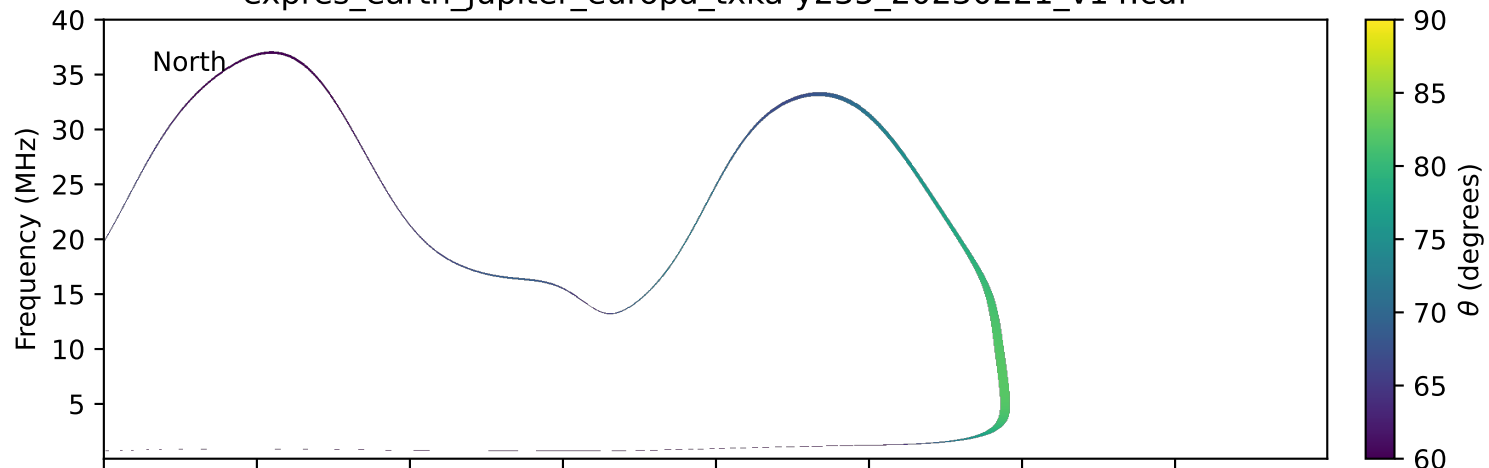
expres_earth_jupiter_europa_txka-y235_20230221_v14.cdf
