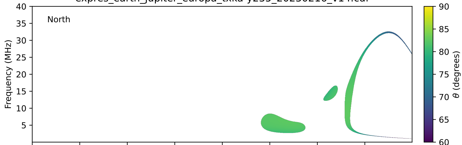
expres_earth_jupiter_europa_txka-y235_20230216_v14.cdf
