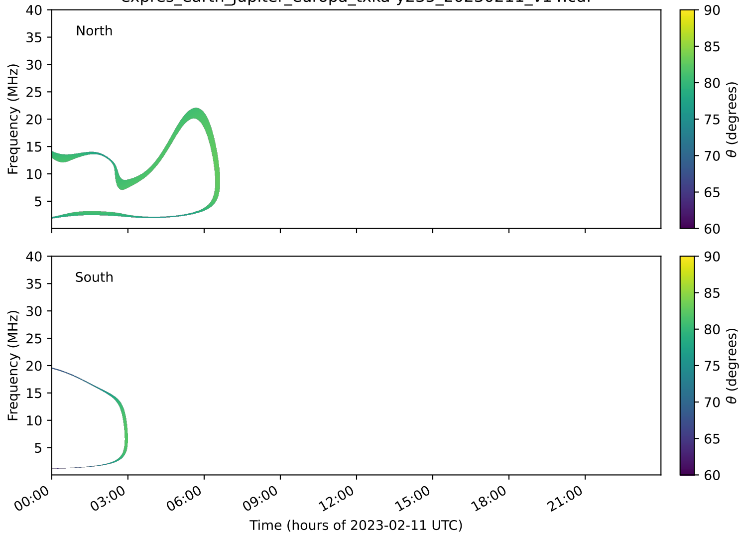
expres_earth_jupiter_europa_txka-y235_20230211_v14.cdf
