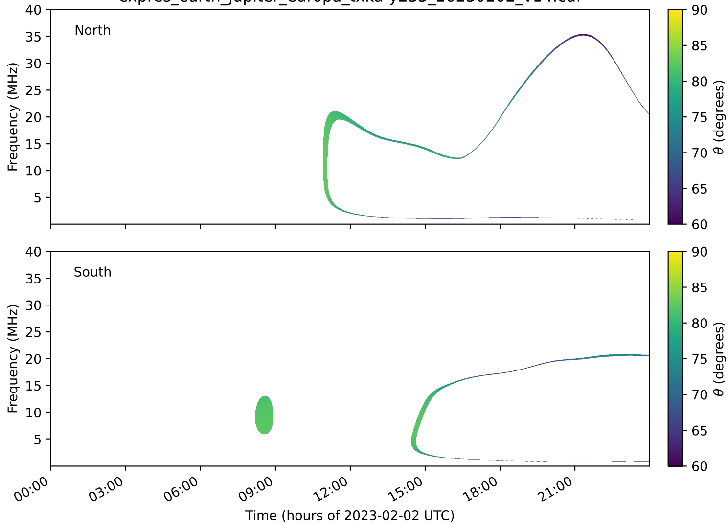
expres_earth_jupiter_europa_txka-y235_20230202_v14.cdf
