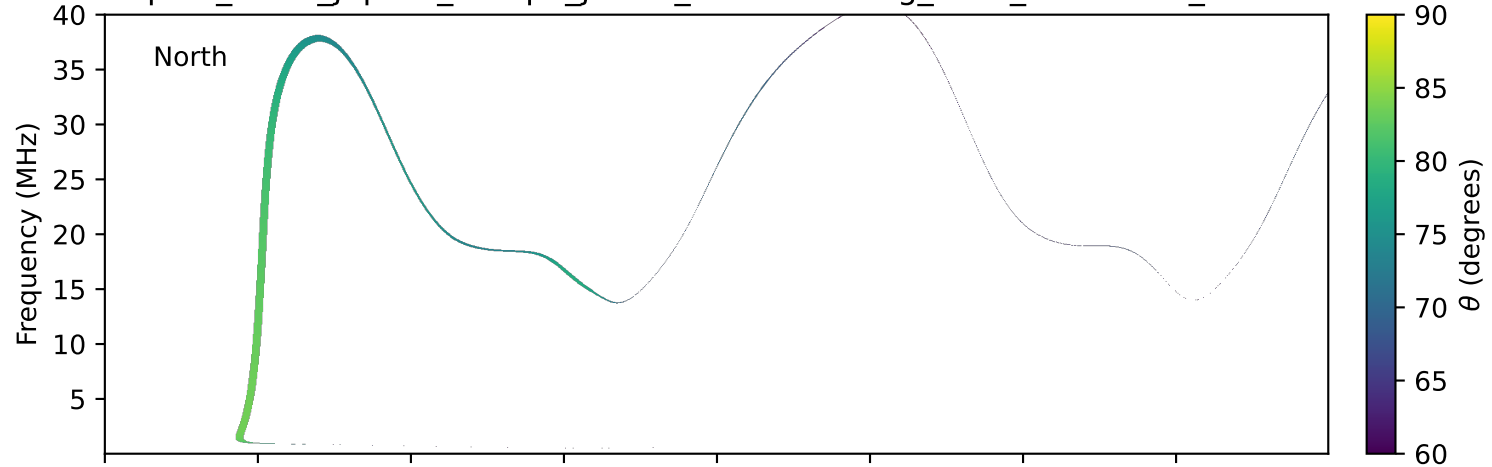
expres_earth_jupiter_europa_jrm33_lossc-wid1deg_3kev_20230206_v11.cdf
