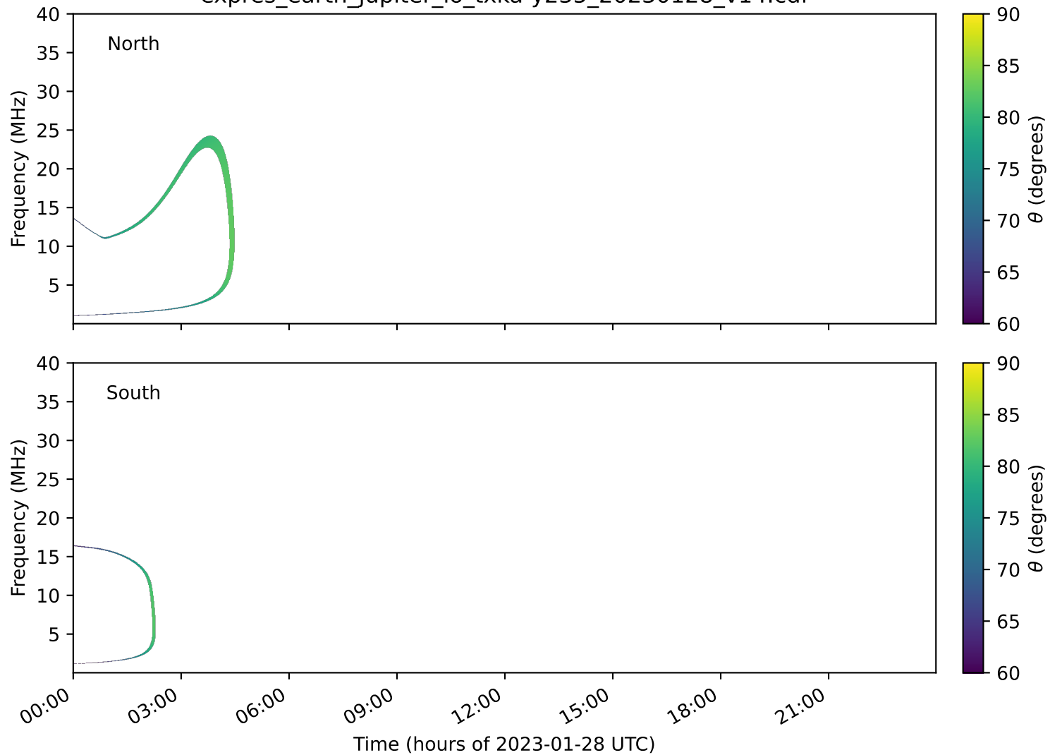
expres_earth_jupiter_io_txka-y235_20230128_v14.cdf
