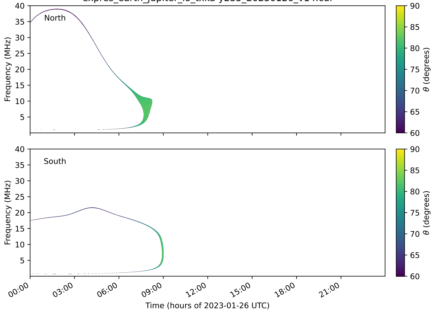
expres_earth_jupiter_io_txka-y235_20230126_v14.cdf
