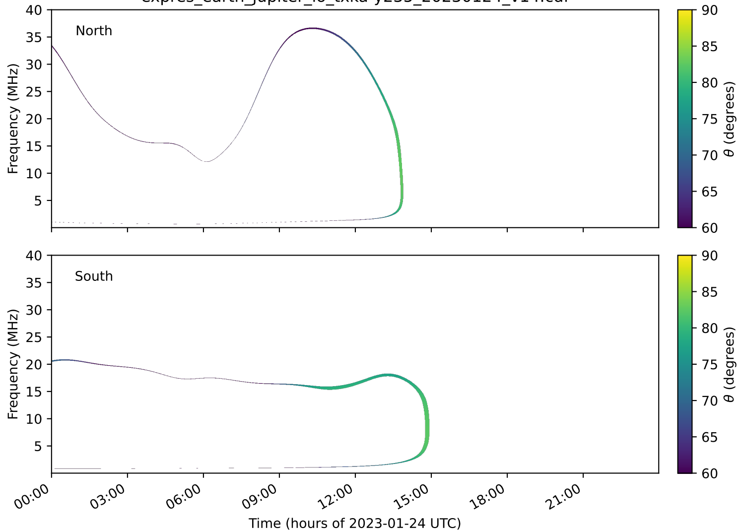
expres_earth_jupiter_io_txka-y235_20230124_v14.cdf
