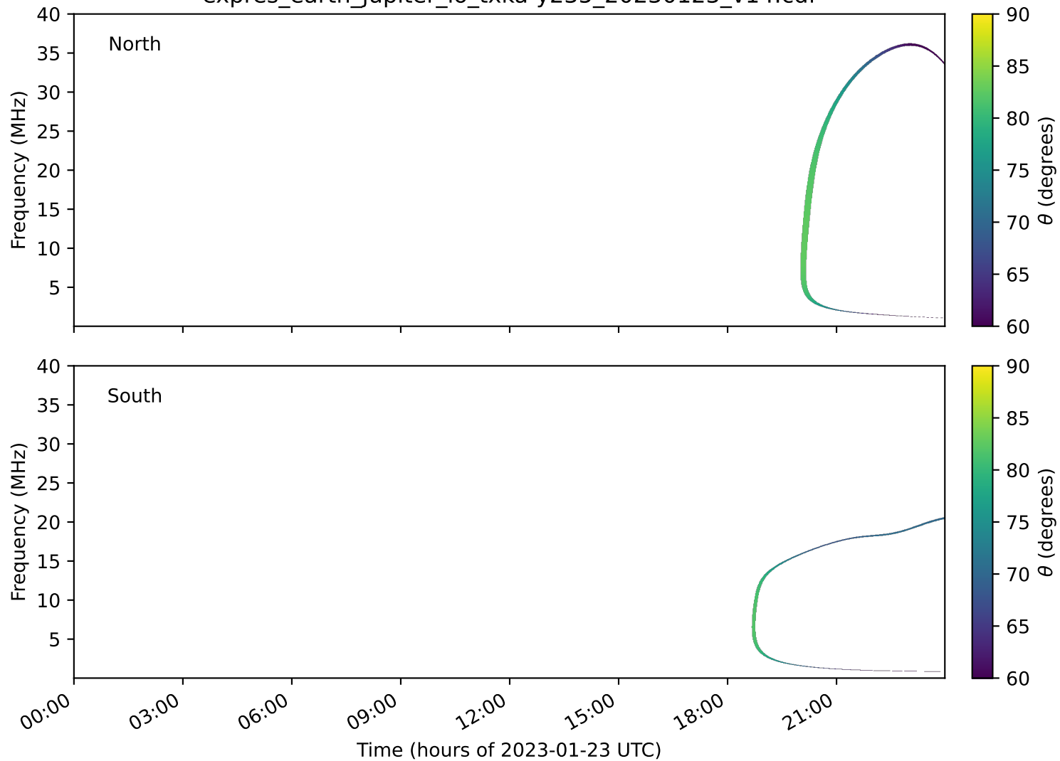
expres_earth_jupiter_io_txka-y235_20230123_v14.cdf
